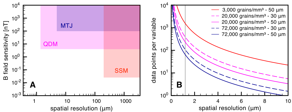
Figure 6. The resolution of the magnetic surface scan. Three potential scanning magnetometry techniques for Micromagnetic Tomography (MMT) have different specifications for spatial resolution and B field sensitivity (a) (with data obtained from Fu et al., 2020; Glenn et al., 2017; Lima et al., 2014; Oda et al., 2016). The theoretically available number of data points per variable that is to be solved by the MMT inversion is governed by the concentration of grains in the sample, the thickness of the sample, and the spatial resolution (i.e., step size) of the magnetic scan (b). The theoretically available number of data points per variable are given for the synthetic sample (3,000 grains/ \text{mm}^3 - 50 \mu\text{m} thick, red line), and different grain concentrations and sample thicknesses for volcanic samples. The typical spatial resolution of the Quantum Diamond Microscope (1.2 \mu\text{m} ) is indicated by the gray line.
